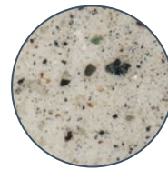
ISO 22/21/18
